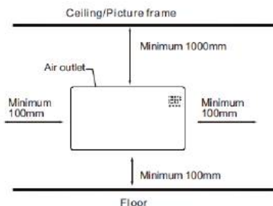
Wall mounted mode
